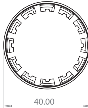
inner cap
